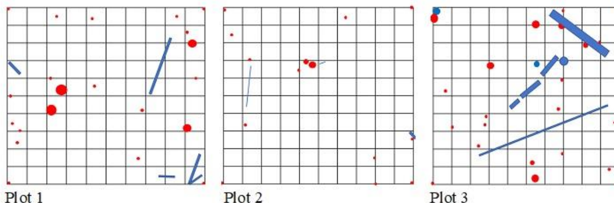
Fig. 2 – Maps of the three plots of the study at the Finca Heimatlos, showing the location of the living trees (red dots), the fallen dead wood (blue rectangular shapes) and stags or stumps (blue dots). The 10 m x 10 m plots are divided into a 100 small squares, each of size 1 m x 1 m. Trees and stags of size 10 cm or more are drawn to scale, but trees of a smaller diameter are shown as same-sized dots.
