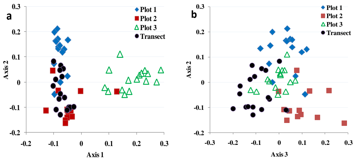
Fig. 4 – Canonical analysis of principal coordinates (CAP) on the species collected during 18 visits to the three plots and the transect between 28 July – 20 Sept 2019; Bray-Curtis similarity calculated using presence-absence data. a Axis 2 vs. Axis 1. b Axis 2 vs. Axis 3.
