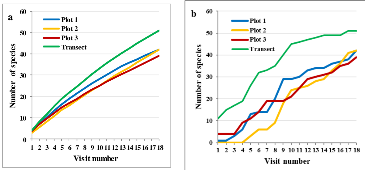
Fig. 3 – Species accumulation curves for the three plots and the transect at Finca Heimatlos. a Randomised. b Non-randomised. i.e. based on the visits in actual order of occurrence.
